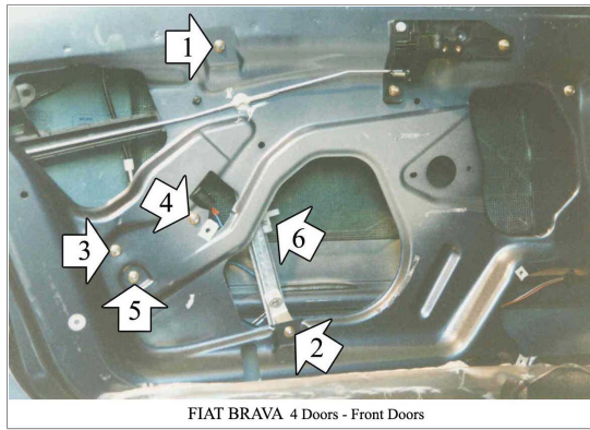
FIAT BRAVA 4 Doors - Front Doors
